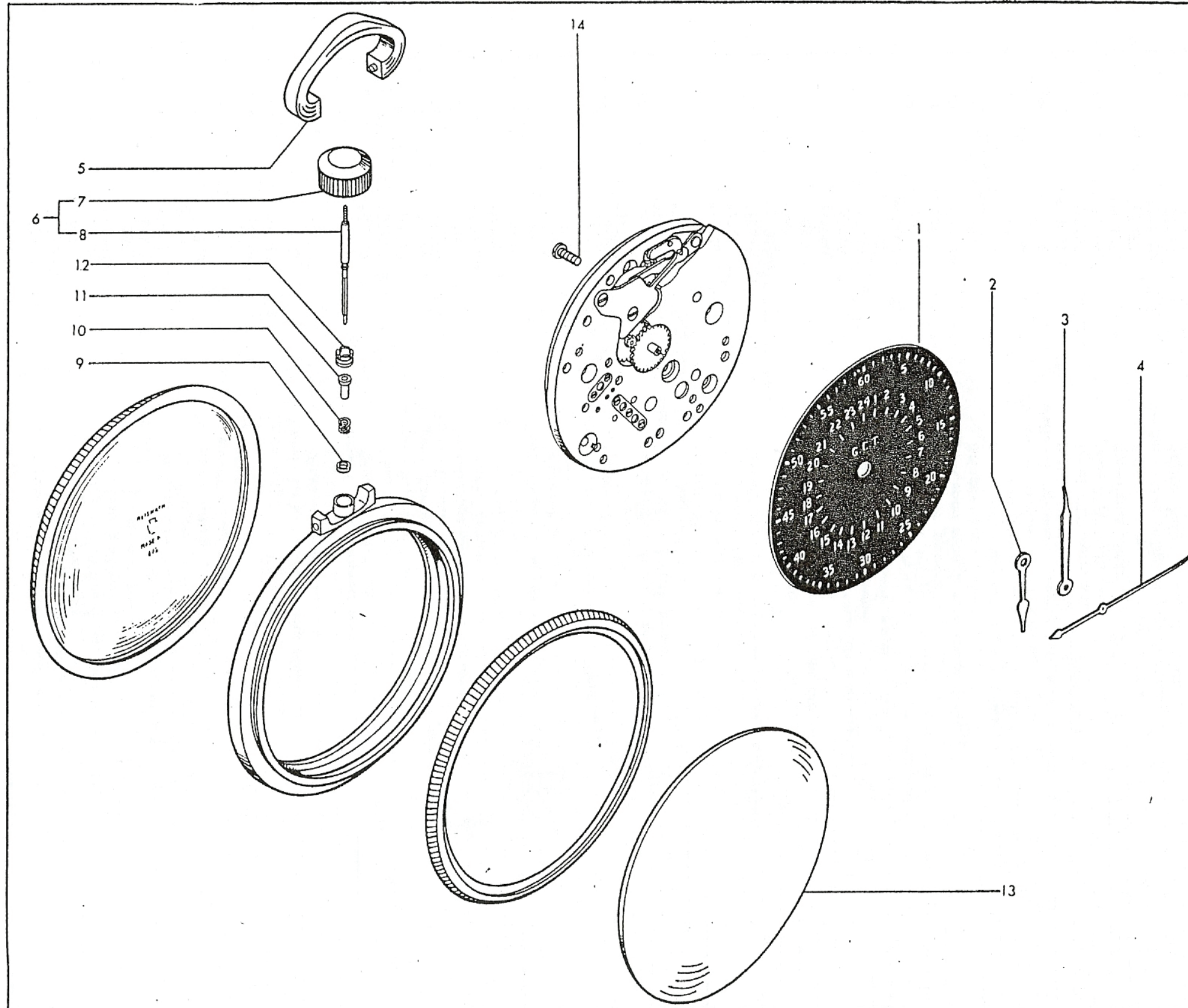
Figure 37 — Exploded View of Component Parts
